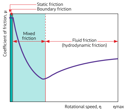
Figure 1. The Stribeck curve: Friction between surfaces as a function of viscosity, speed and load.
